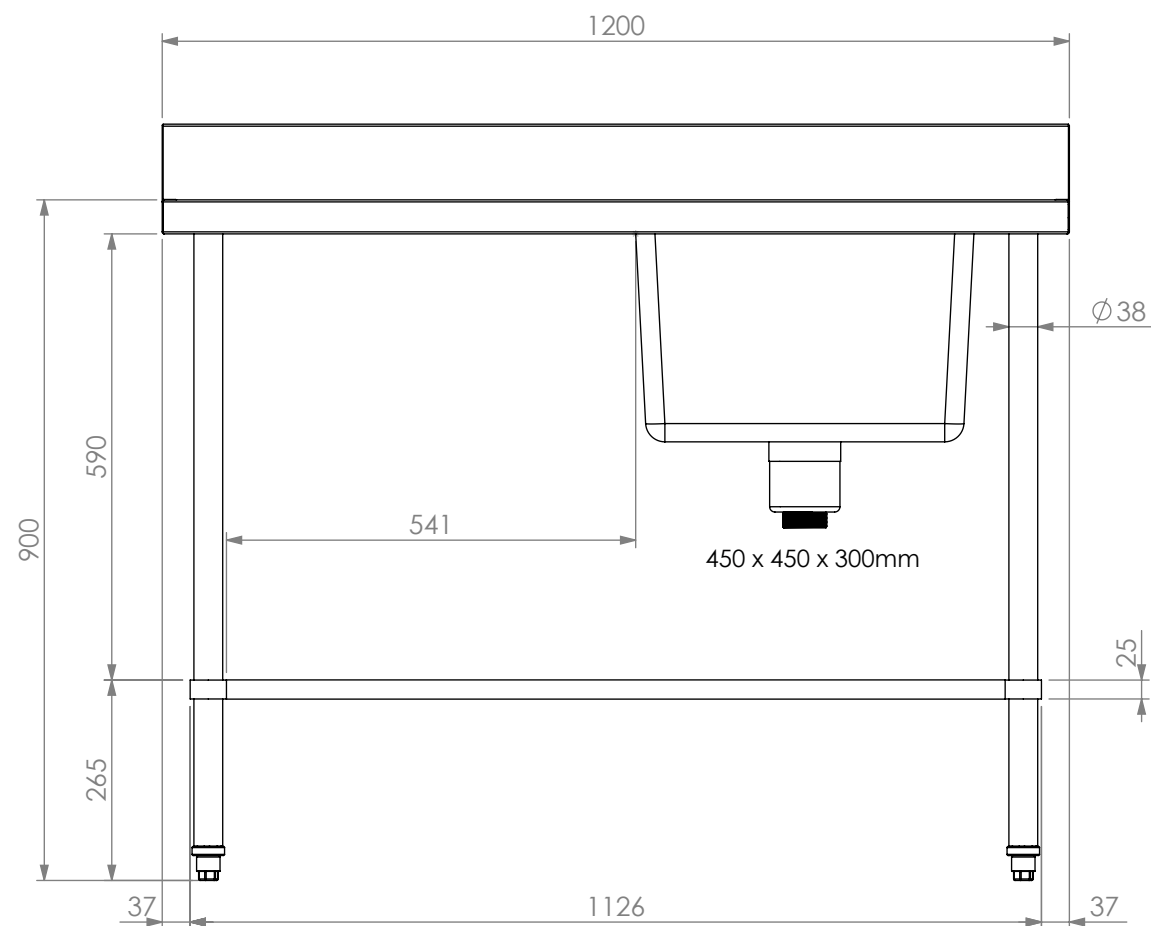
FRONT ELEVATION
